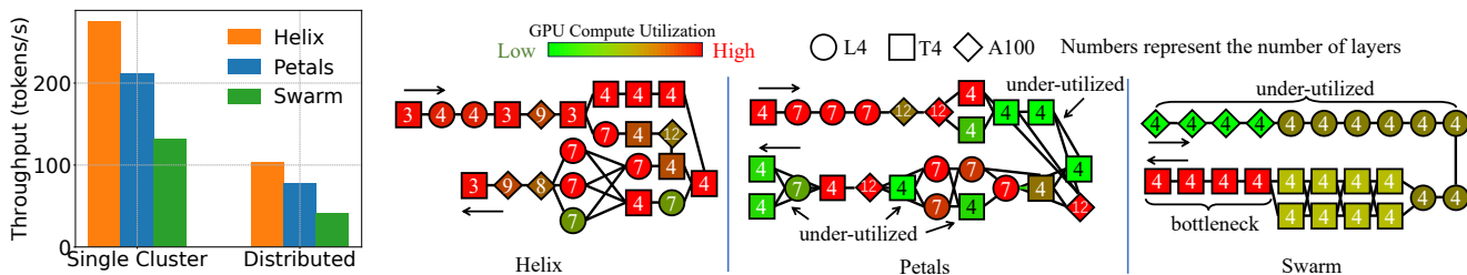
Figure 10: Left: decode throughput of Helix, Petals and Swarm in single and distributed cluster setup. Right: A case study of the model placement found by the three methods for serving LLaMA 70B in single cluster setup. The number in each node represents the number of layers the node holds.
