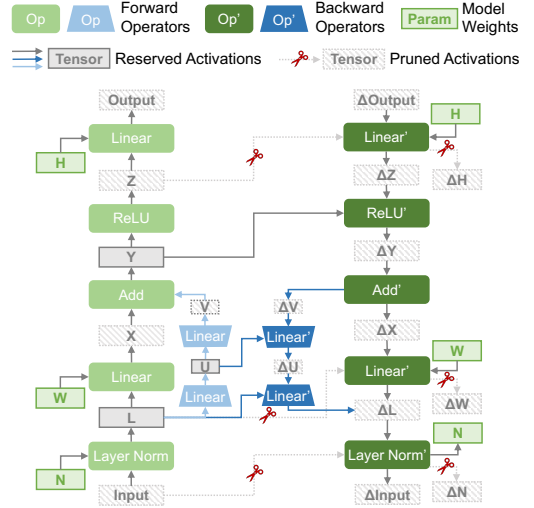
Figure 5: Static graph pruning for an MLP model with LoRA.
