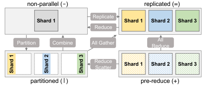
Figure 3: Four possible parallel states for a tensor dimension and their transitions. For each parallel state, the symbol in parenthesis shows the notation FlexLLM used to represent it.
