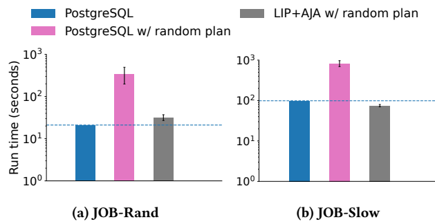
Figure 9: Performance of LIP+AJA on JOB-Rand and JOB-Slow with random input query plans.
