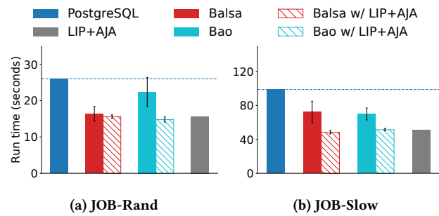
Figure 8: Applying LIP+AJA to plans from Balsa and Bao.
