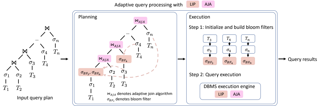
Figure 4: Overview of adaptive query processing with LIP+AJA.
